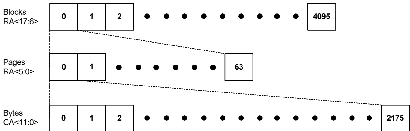
Figure 1-4. Memory Mapping Diagram for AS5F34G04SND-08LIN, AS5F14G04SND-10LIN
