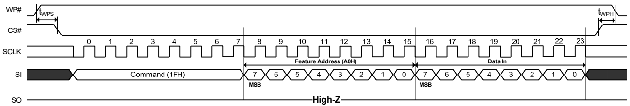
Figure 16-4. WP# Timing
