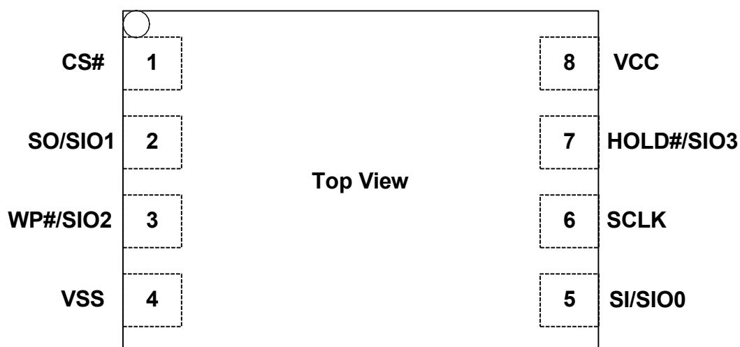
Figure 1-6. Pin Assignments
