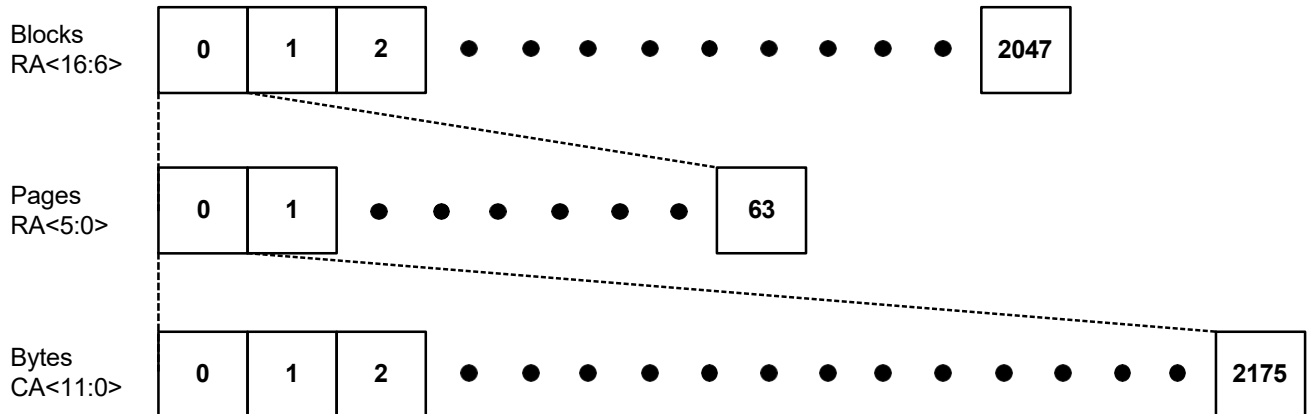
Figure 1-3. Memory Mapping Diagram for AS5F32G04SND-08LIN, AS5F12G04SND-10LIN
