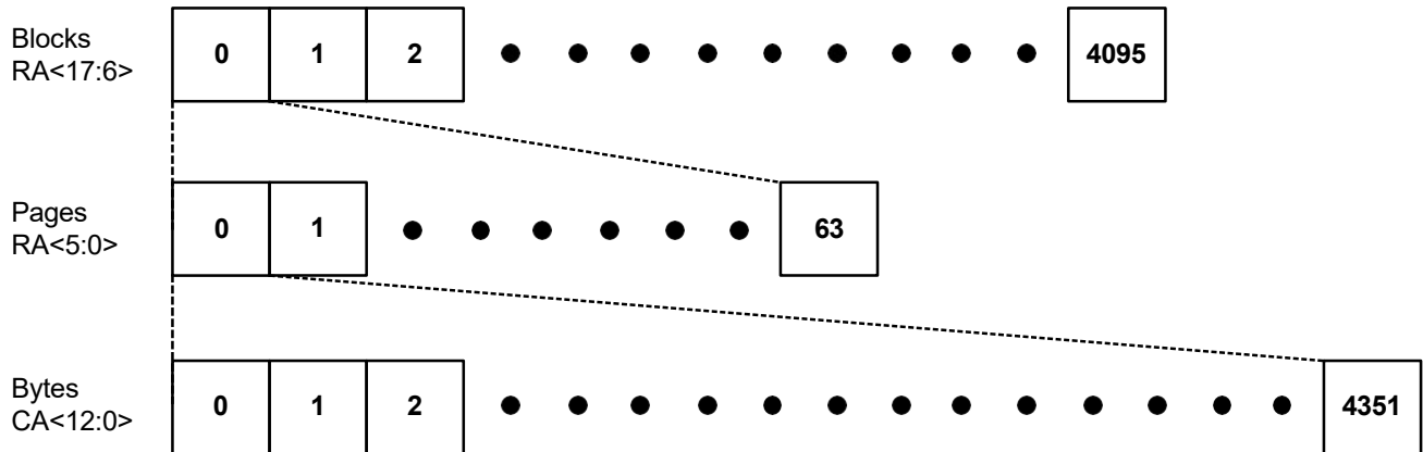
Figure 1-5. Memory Mapping Diagram for AS5F38G04SND-08LIN, AS5F18G04SND-10LIN
